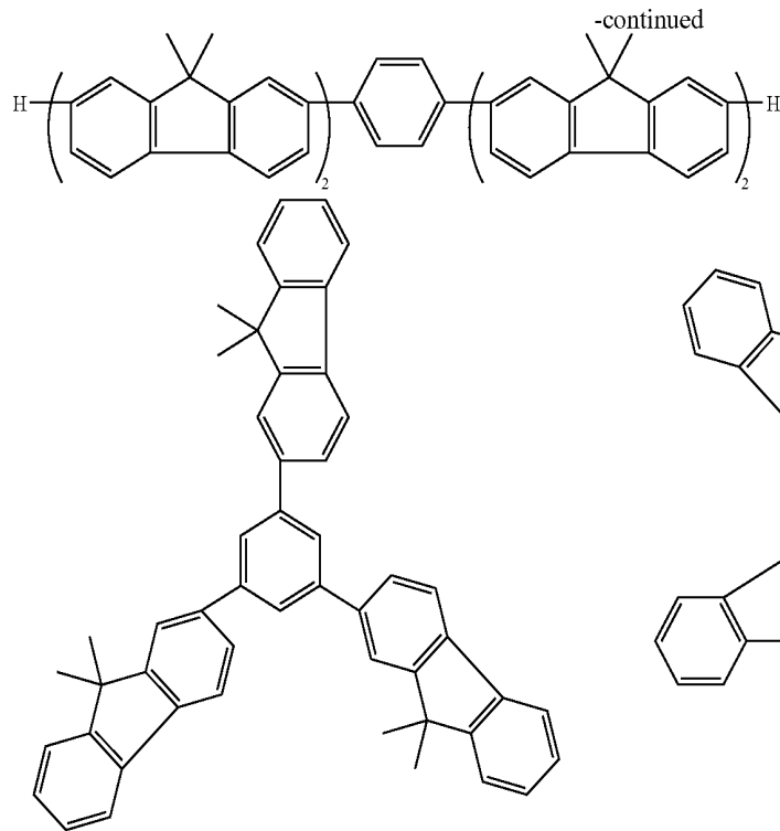
Compound Having Fluorene Ring and Pyrene Ring
