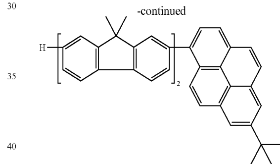
Compound Having Fluorene Ring and Pyrene Ring
